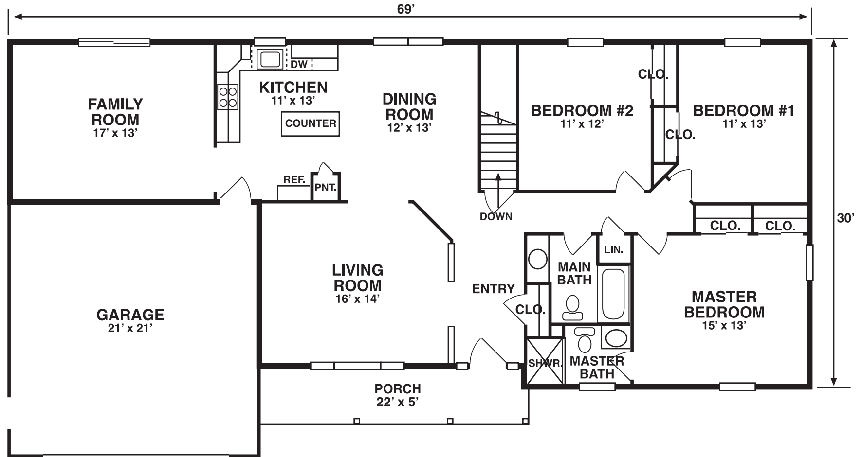
MAIN LEVEL
