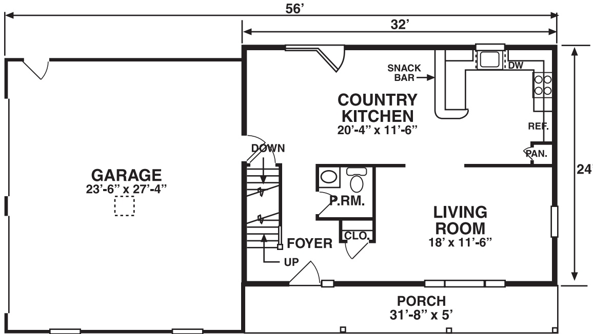
FIRST FLOOR
